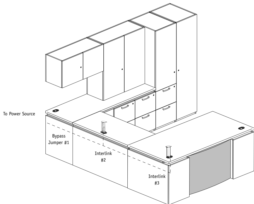
Interlink System shown using a bypass jumper for position 1, connecting to the power source and then 2 interlink modules; specify NACELILJ1, NACELIL2, and NACELIL3
