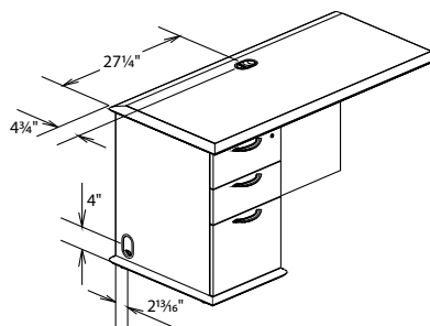
Executive Return (Box/Box/File or File/File) Center grommet on worksurface and grommet on end panel (36N2553RLEFW1 Shown)
