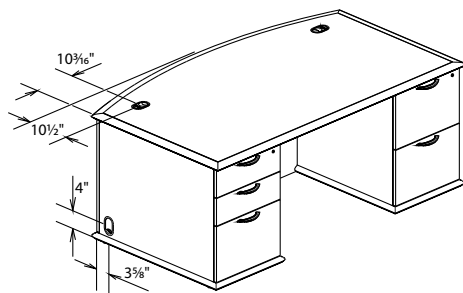
Single and Double Pedestal Arc Top Desks Grommets on worksurface and end panels (36N3773DDFAW8 Shown)
