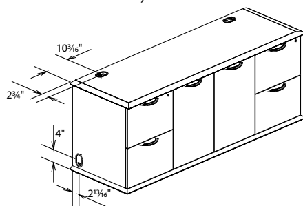
Storage Credenza and Single Pedestal Credenza Grommets on worksurface and end panels (36N2473CSFW2 Shown)
