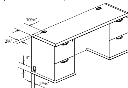
Kneespace Credenza Grommets on worksurface and end panels (36N2473CKFW2 Shown)
