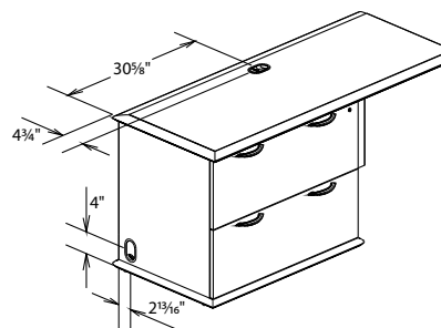
Executive Return (Lateral File) Center grommet on worksurface and grommet on end panel (36N2559RLEFW6 Shown)
