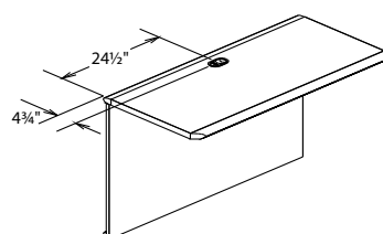
Bridge Center grommet on worksurface (36N2551BEFW Shown)
